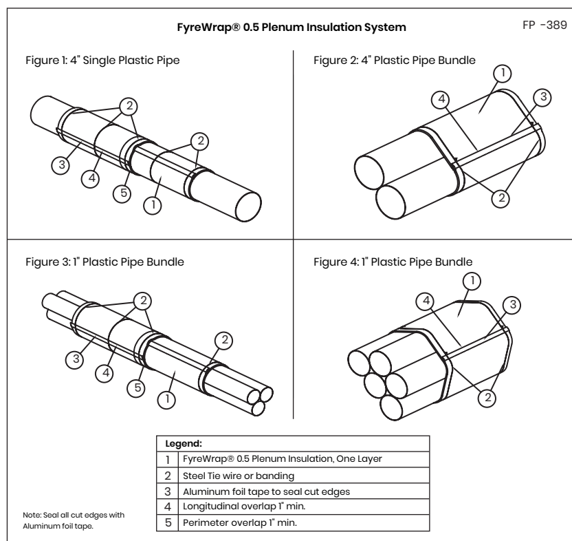
Figure 1. Installation Detail
