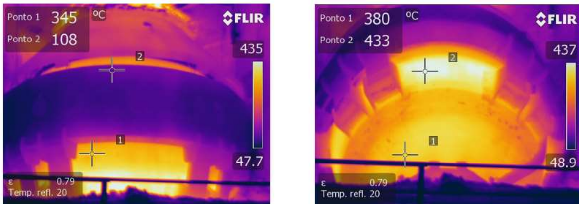
Figure 9 – Thermography performed on BOF with 400 heats.
