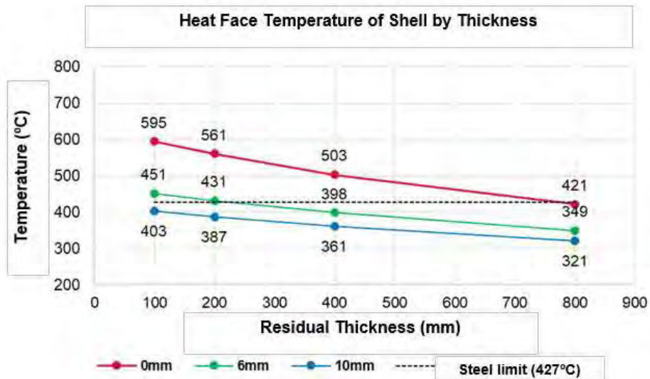
Figure 8 – Evaluation of final shell temperature as a function of residual thickness.
