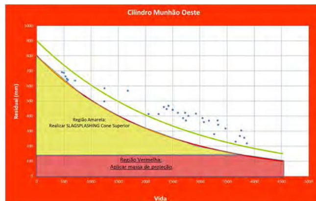
Figure 11. Trunnion wear curve.
