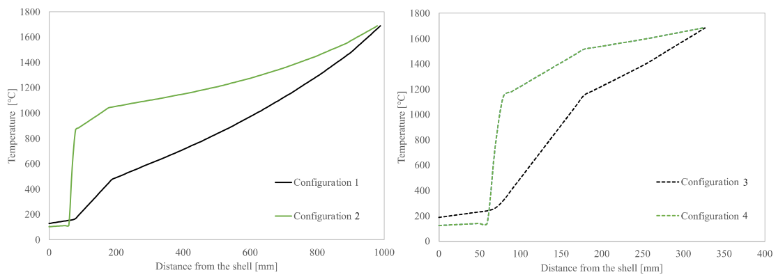
Figure 7 – Thermal profile along the material
