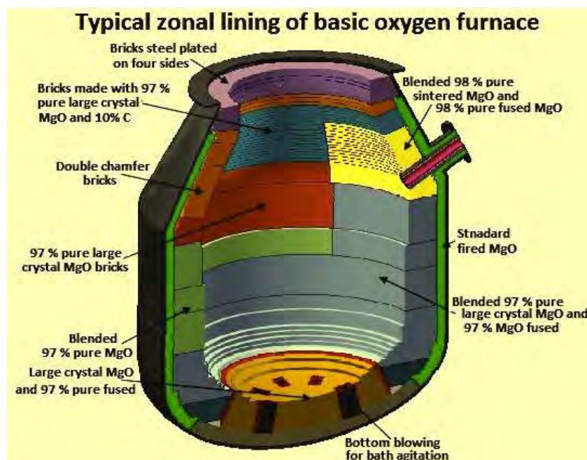
Figure 1 - Schematic representation of the converter (5)
