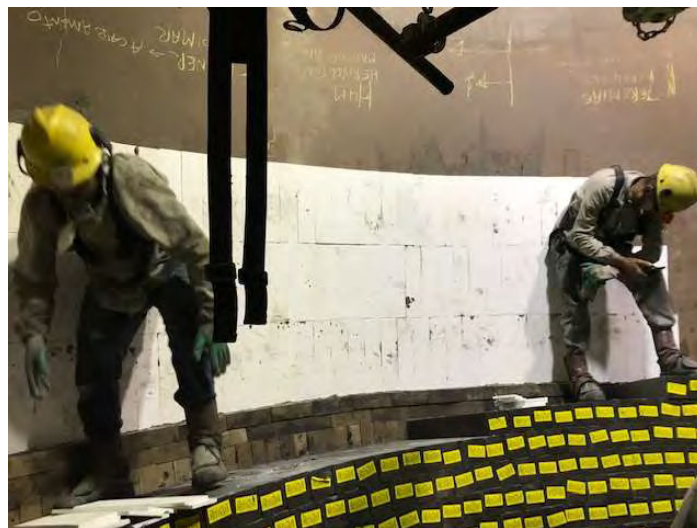
Figure 3. Installation of the thermal insulation in the Cylinder of BOF#4.
