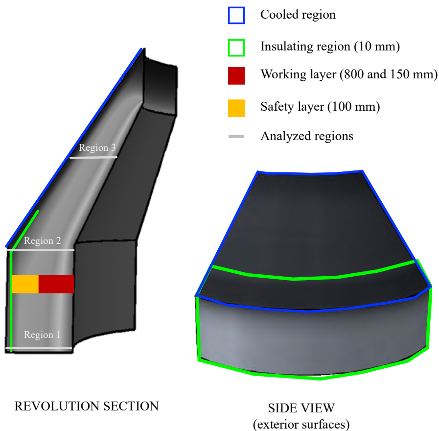
Figure 2: Cross-section and lateral view of the studied problem.
