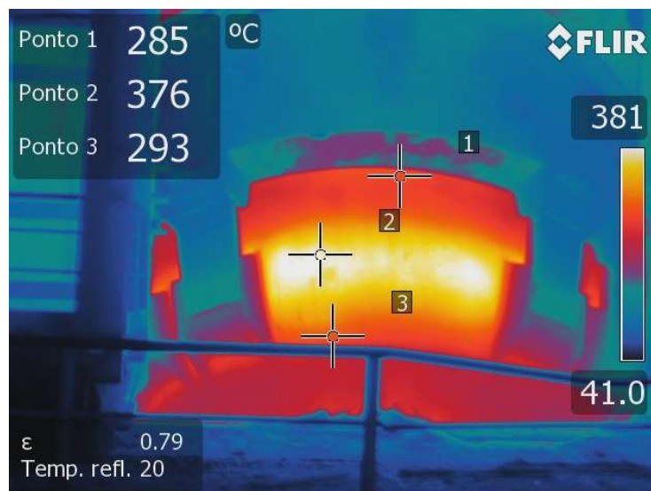
Figure 10 – Thermography of BOF#4 with 4000 heats.
